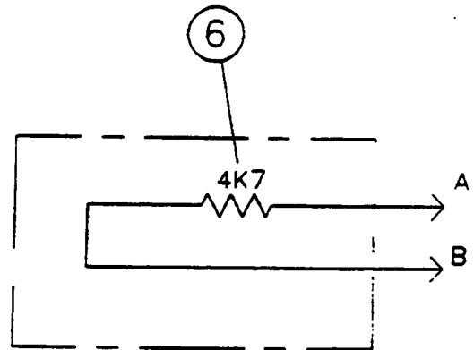
WIRING DETAIL
